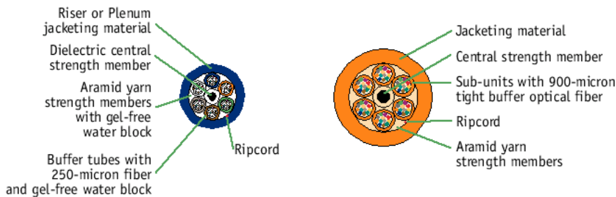
72 fiber ADVENTUM Outdoor/Indoor Cable
